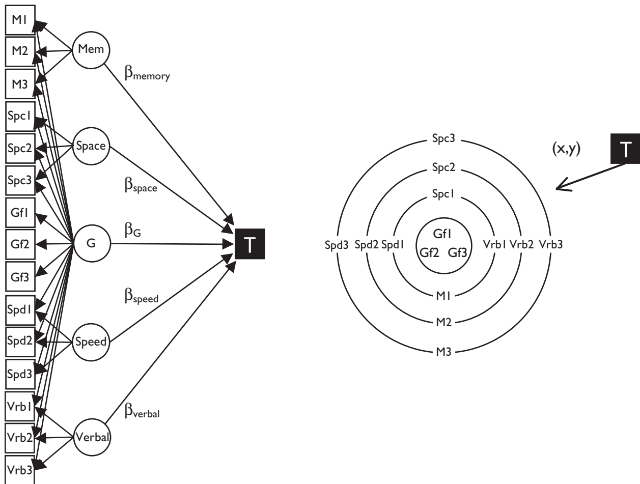
Figure 1. Left: examining the meaning of target variable "T" in the context of a well-established factor structure. Right: examining the meaning of target variable "T" in the context of a well-established radex solution.
