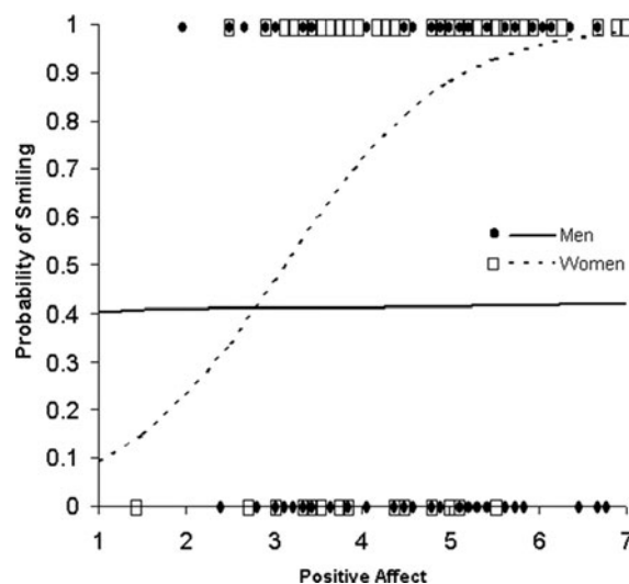
Figure 1 (Vazire et al.). Men's and women's probability of smiling as a function of positive affect. This plot is based on the results of two separate binary logistic regressions (one for men and one for women) predicting smiling from positive affect. The x-axis represents the possible range of positive affect scores, and the y-axis represents probability of smiling based on the results of the regressions. The individual dots represent data from individual men (circles) and women (squares) who did and did not smile. Smiling was coded as a binary variable, so the dots appear on the y = 0 and y = 1 lines.
